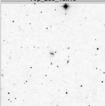
Arp_237_15x15
