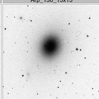
Arp_134_15x15
