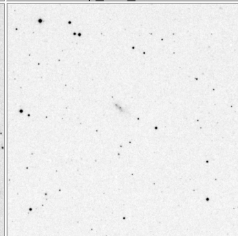
Arp_267_15x15
