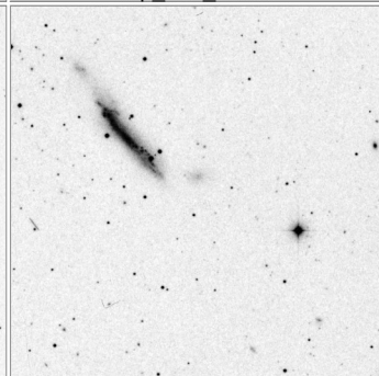
Arp_206_15x15
