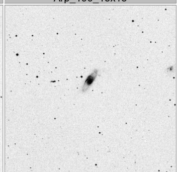
Arp_200_15x15
