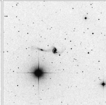
Arp_284_15x15
