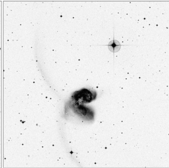
Arp_244_15x15
