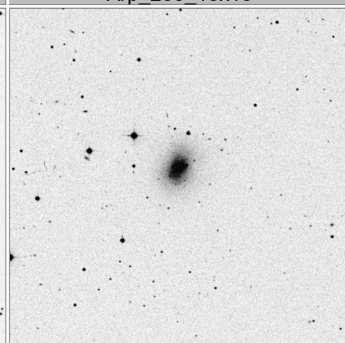
Arp_234_15x15
