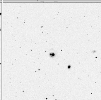
Arp_236_15x15
