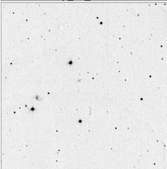
Arp_45_15x15
