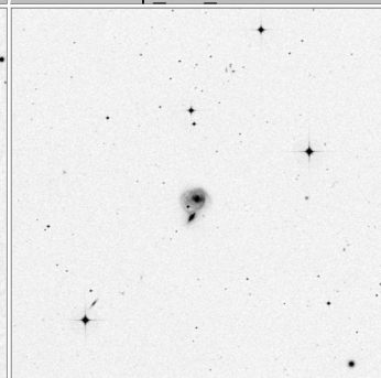
Arp_127_15x15
