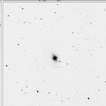
Arp_230_15x15
