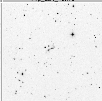
Arp_238_15x15
