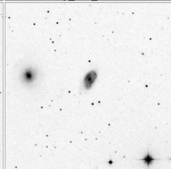
Arp_227_15x15
