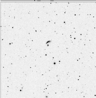
Arp_125_15x15
