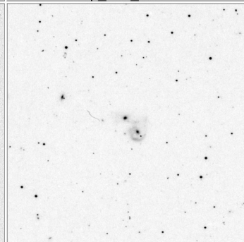
Arp_107_15x15
