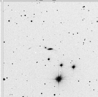
Arp_287_15x15
