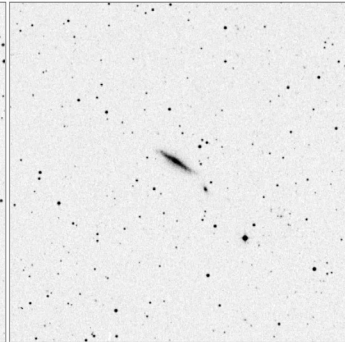
Arp_124_15x15
