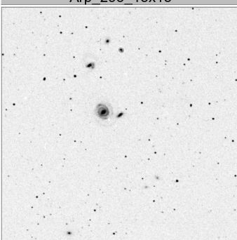
Arp_297_15x15
