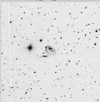
Arp_273_15x15
