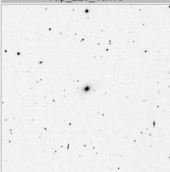
Arp_233_15x15
