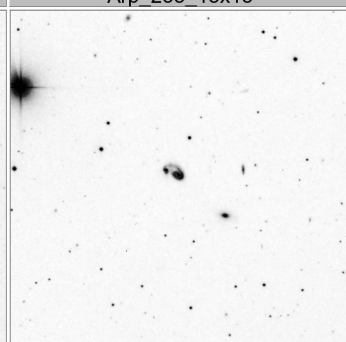
Arp_239_15x15
