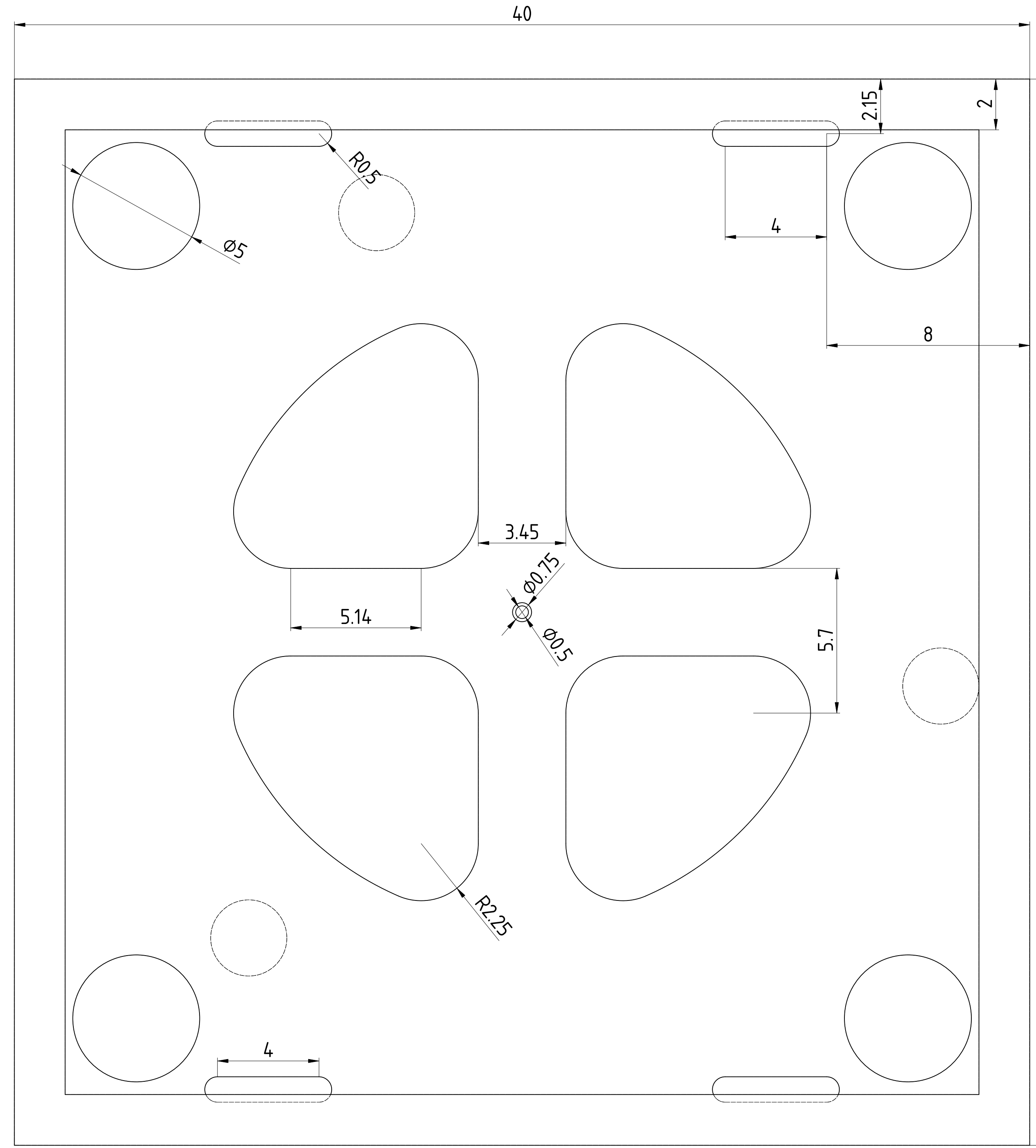
Top View
